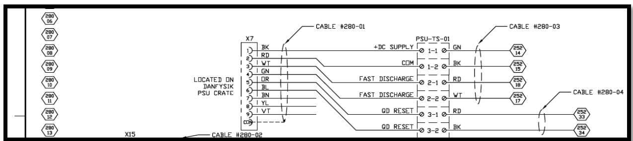
Fig.1. Upper section of drawing A00000-16-03-0280 Power Supply Crate Connections Wiring Diagram
